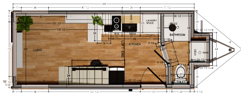
MAIN FLOOR AREA
